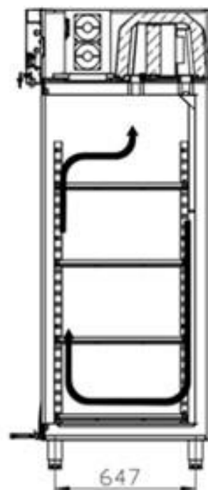
SECTION I-I
