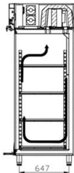
SECTION I-I
