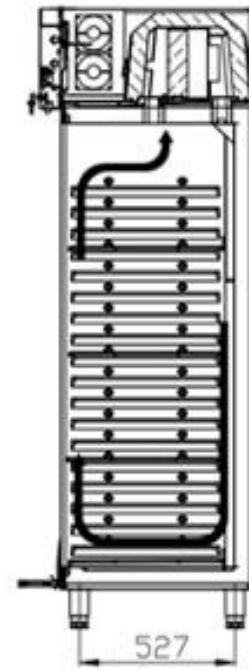
SECTION G-G
